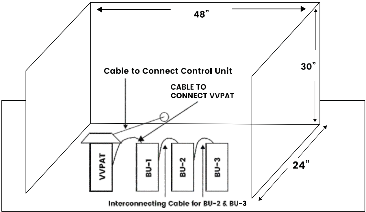
CASCADING OF THREE BALLOT UNITS
